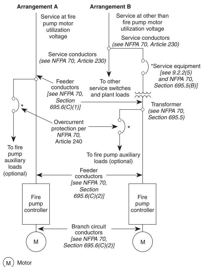
FIGURE A.9.3.2 Typical Power Supply Arrangements from Source to Motor.
