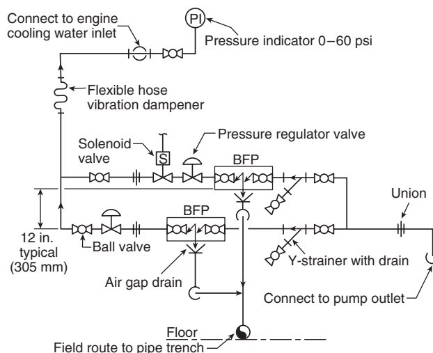
FIGURE A.11.2.8.5.3.7(B) Backflow Preventer Arrangement.
