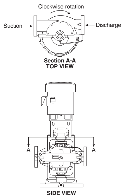
FIGURE A.4.23(b) Vertical Pump Shaft Rotation.
