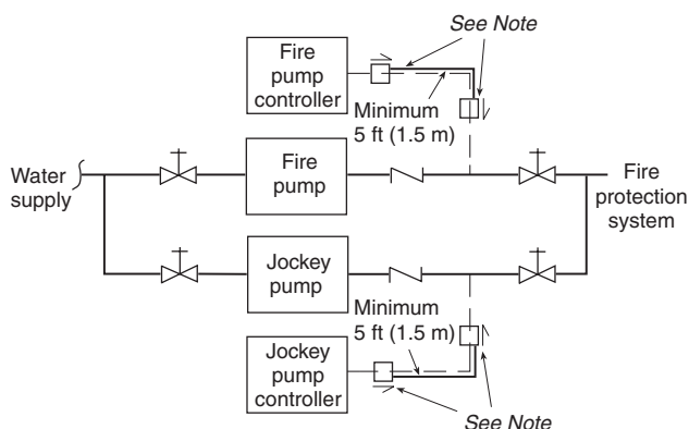
FIGURE A.4.30(b) Piping Connection for Pressure-Sensing Line (Diesel Fire Pump).
