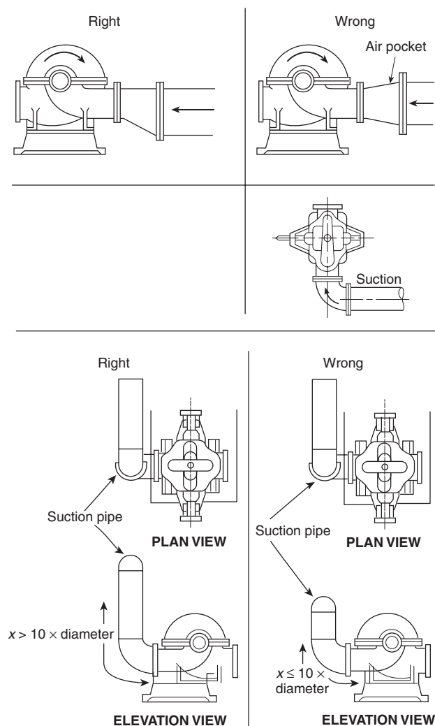
FIGURE A.4.14.6 Right and Wrong Pump Suctions.
